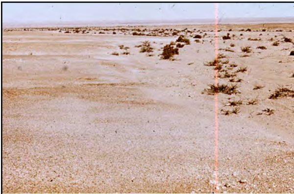
No.20, Gypsic Yermosol, Petrogypsic Gypsiorthid, in Namib desert
